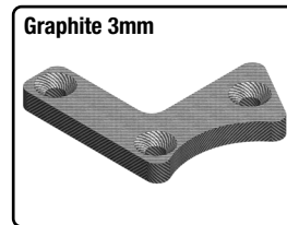
Graphite 3mm C-00180-235 Suspension arm stiffener - B - Lower Front - Left - 1 pc
