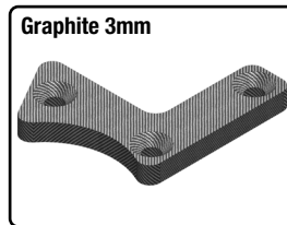
Graphite 3mm C-00180-234 Suspension arm stiffener - B - Lower Front - Right - 1 pc
