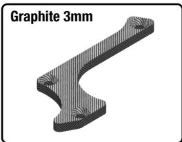
Graphite 3mm C-00180-232 Suspension arm stiffener - A - Lower Front - Right - 1 pc
